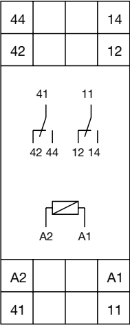
CR-M2SS, CR-M2SF
