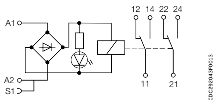
RB (R) 122G-24VUC/48-60VUC
