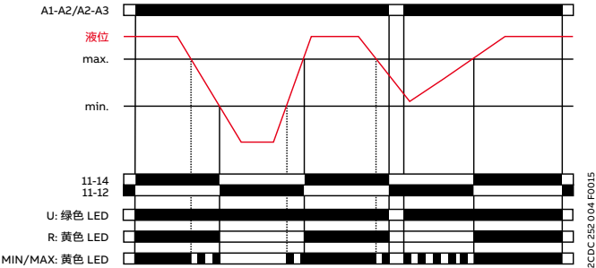
抽干: CM-ENS.1x, CM-ENS.2x
