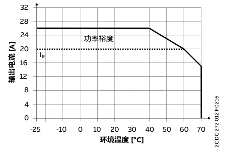
CP-C.124/20.0, CP-C.124/20.0-L
