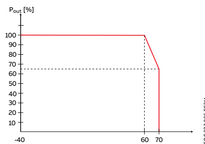
CP-T 24/40.0, CP-T 48/20.0
