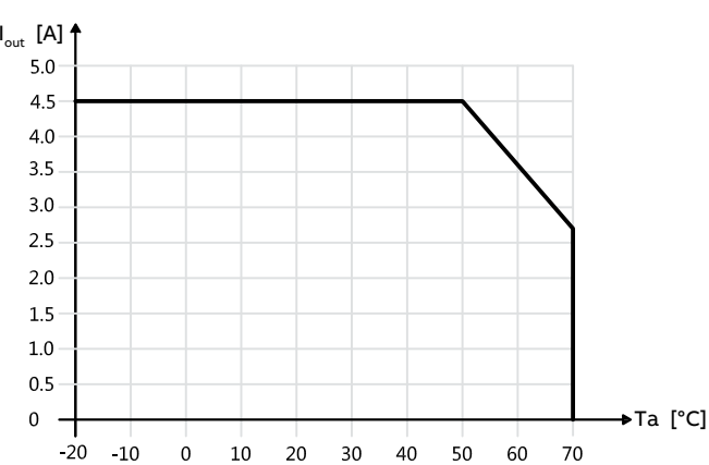
CP-PX 24/4.5
