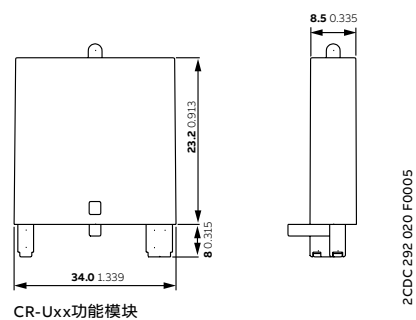
CR-Uxx功能模块
