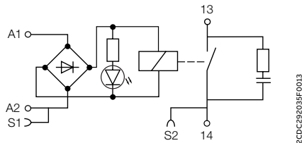
RB (R) 111R-24VUC
