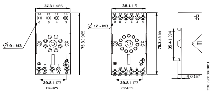
CR-U2S - CR-U3S - 螺钉连接
