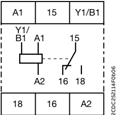
CT-MFD.12
