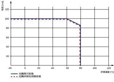
CR-S晶体管输出降容曲线
