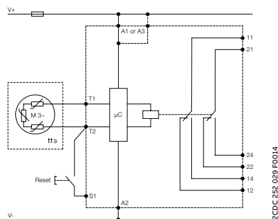
CM-MSS.33x
