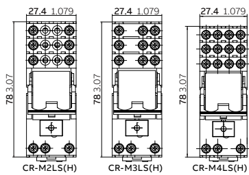
CR-M2LS(H) - CR-M3LS(H) - CR-M4LS - 螺钉连接
