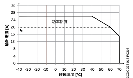
CP-C.124/20.0-C
