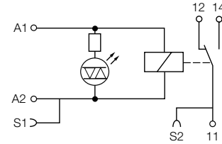
RB (R) 121-12VDC/24VDC
