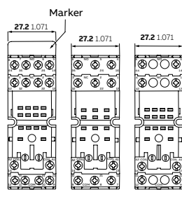
CR-M2SS - CR-M3SS - CR-M4SS - 螺钉连接
