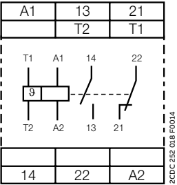
CM-MSS.11x, CM-MSS.21x
