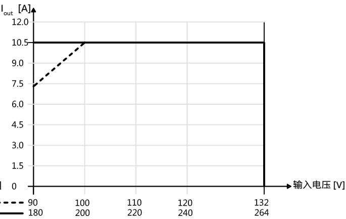
CP-PX 24/10.5
