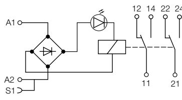
RB (R) 122G-115VUC/230VUC
