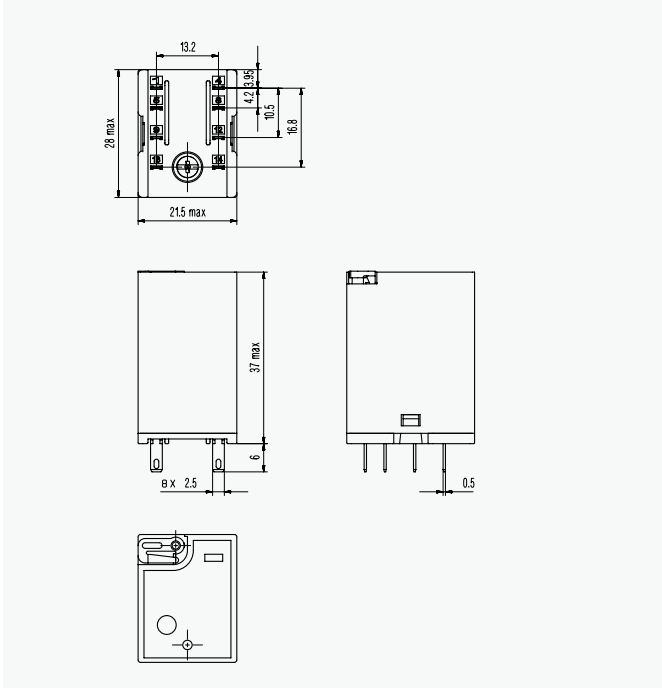
CR-MX, 2 c/o (SPDT) 触点, 带测试按钮
