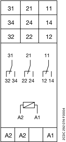
CR-M3LS(H)
