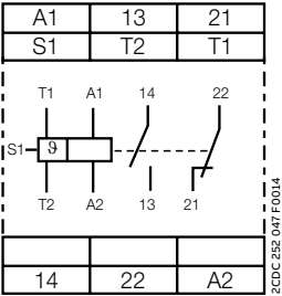
CM-MSS.31x
