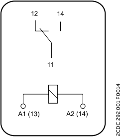
CR-S
