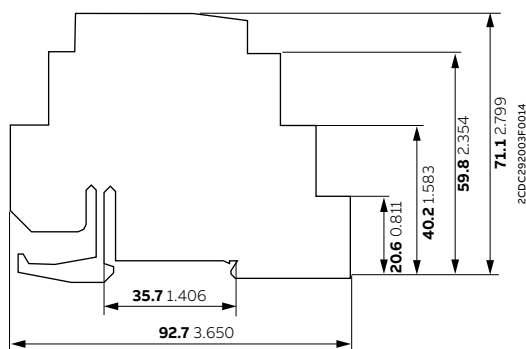
CR-S隔板
