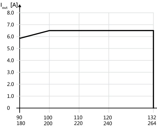
CP-PX 24/14.6
