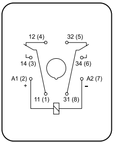
CR-U, 2 c/o触点
