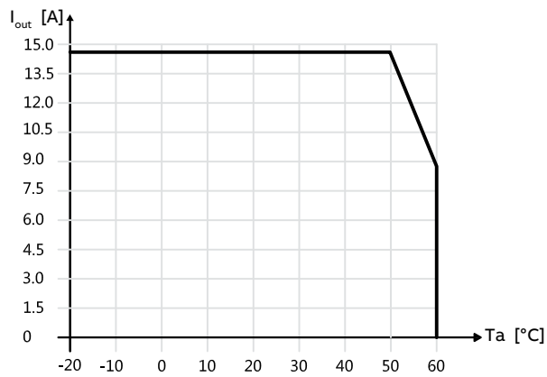
CP-PX 24/14.6
