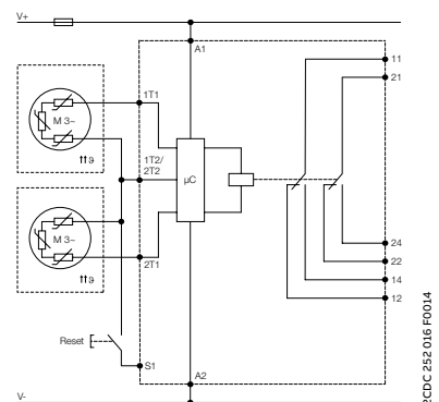
CM-MSS.51x
