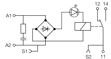
RB (R) 121R-115VUC/230VUC
