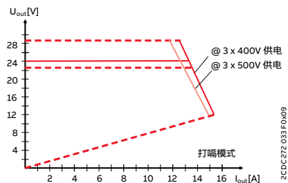
CP-T 24/10.0
