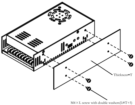
M4×L screw with double washers(L=T+5)
