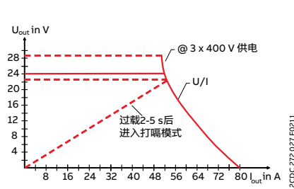
CP-T 24/40.0
