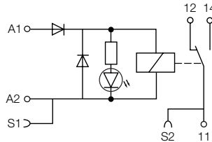
RB (R) 121P (G) -5VDC/12VDC
