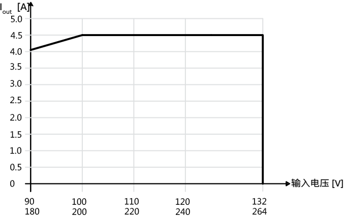
CP-PX 24/4.5
