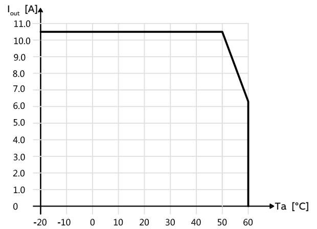
CP-PX 24/10.5
