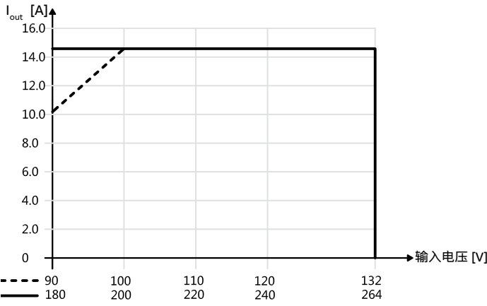
CP-PX 24/14.6
