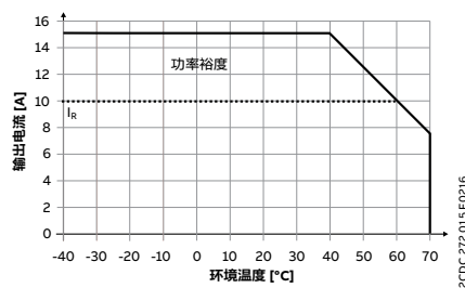
CP-C.124/10.0-C
