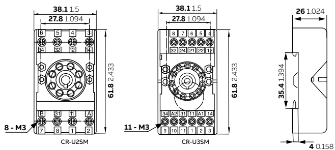
CR-U2SM - CR-U3SM - 螺钉连接
