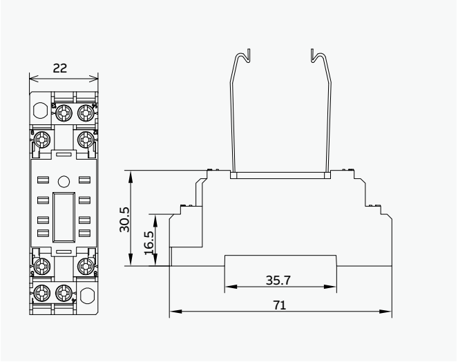
CR-M2SFBN
