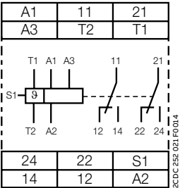
CM-MSS.23x, CM-MSS.33x
