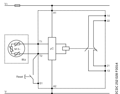
CM-MSS.31x
