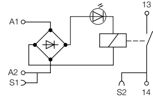
RB111-115VUC/230VUC
