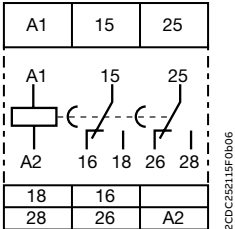
CT-ERD.22
