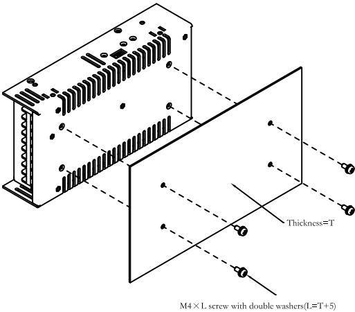
M4×L screw with double washers(L=T+5)
