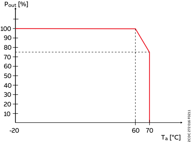
CP-E 5/3.0, CP-E 24/0.75
