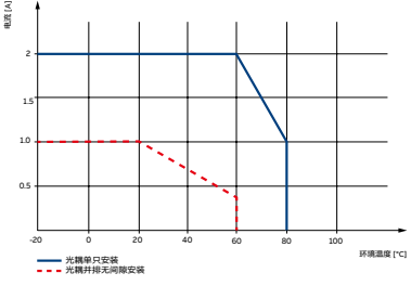
CR-S Triac输出降容曲线
