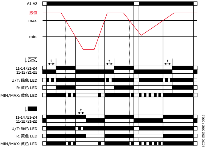
抽干: CM-ENS.31
