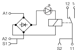
RB (R) 121 (G) -48-60VUC/ 115VUC/230VUC/60-230VUC
