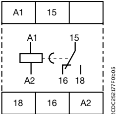
CT-ERD.12
