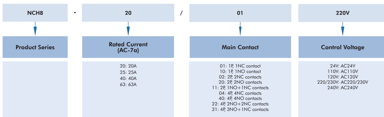
NCH8 Contactor 20~63A
